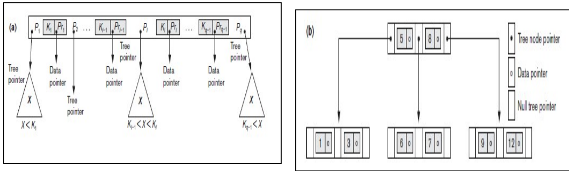
Figure 6.24: sample B tree
