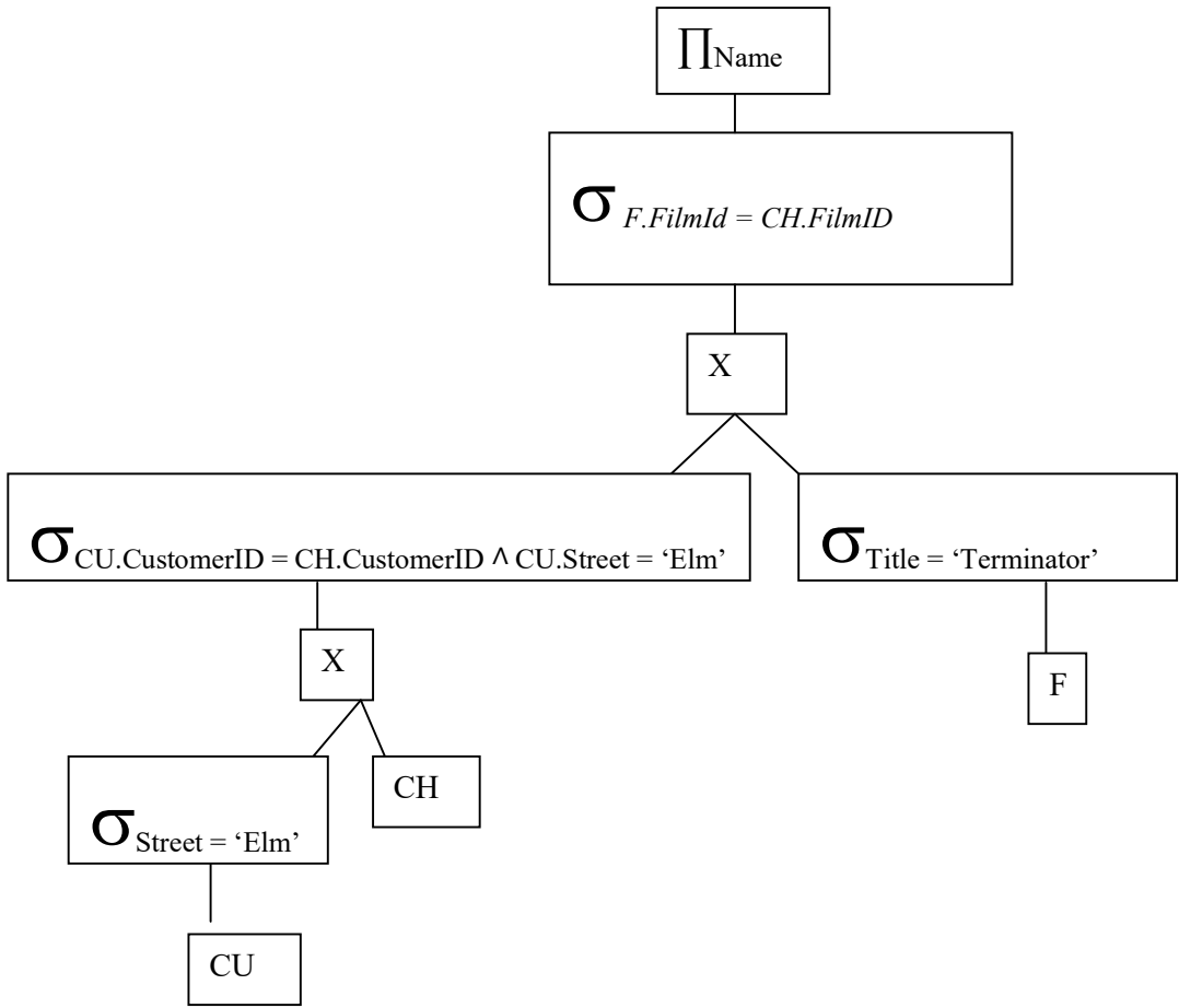
Figure 5.3: Query using applying selection early
