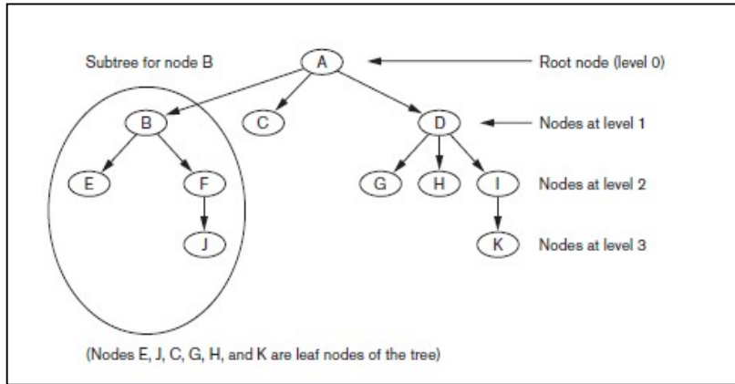
Figure 6.21: Tree data structure
