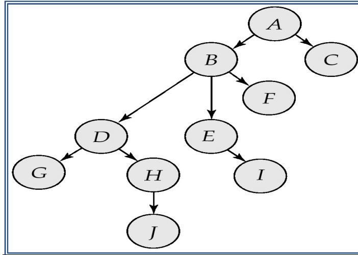
Figure 5.21: Example of Tree protocol
