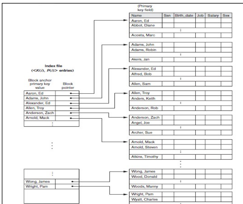
Figure 6.15: Sample Index file
