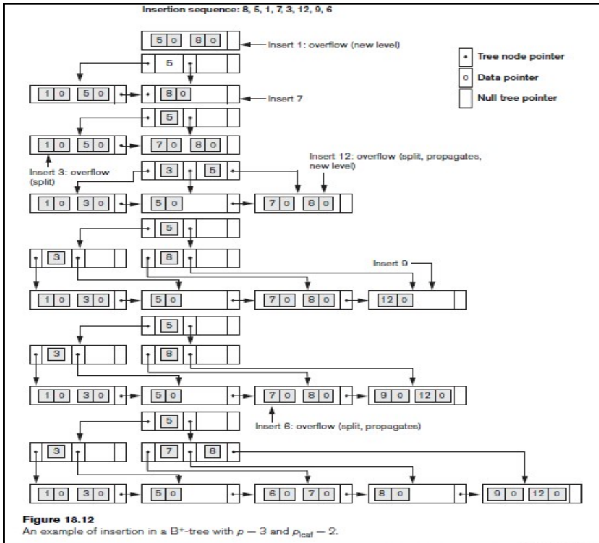
Figure 6.26: Insertion in B+ tree
