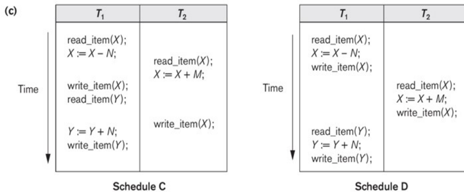
Figure 5.11: Examples of non-serial schedules
