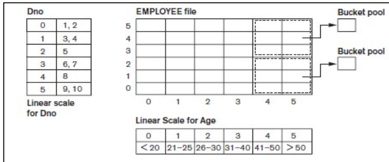
Figure 6.28: Sample Grid file
