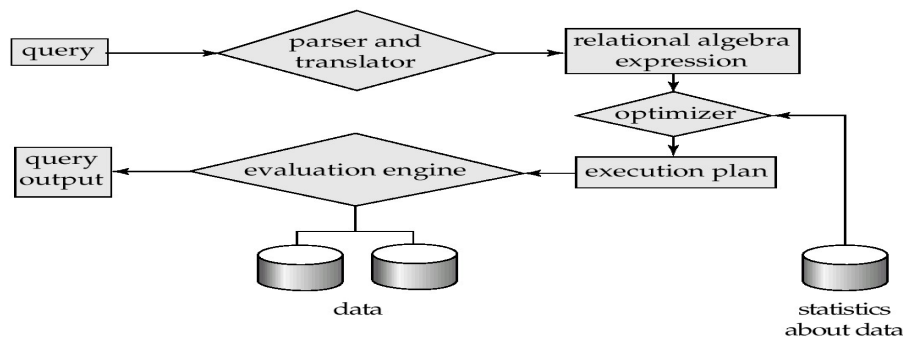
Figure. 5.1: Query processing
