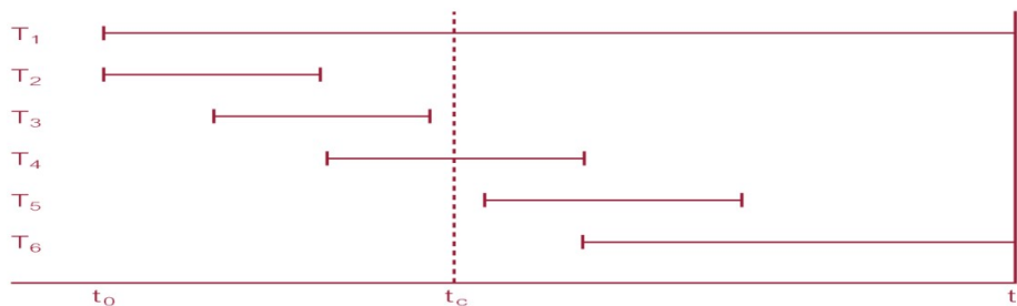
Figure 5.28: Example of Recovery
