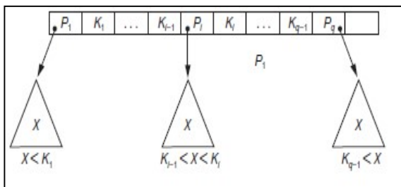
Figure 6.22: Sub tree
