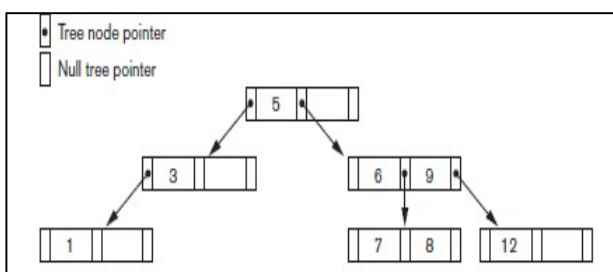
Figure 6.23: Sub tree
