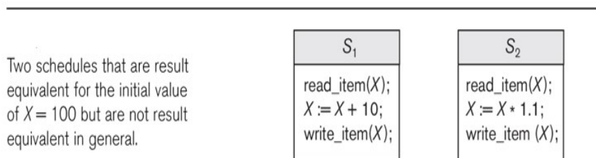
Figure 5.12: Examples of equivalent schedules
