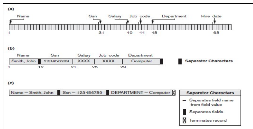
Figure 6.5: File separator
