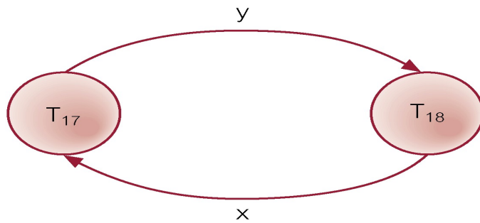
Figure 5.24: Wait-For-Graph (WFG)
