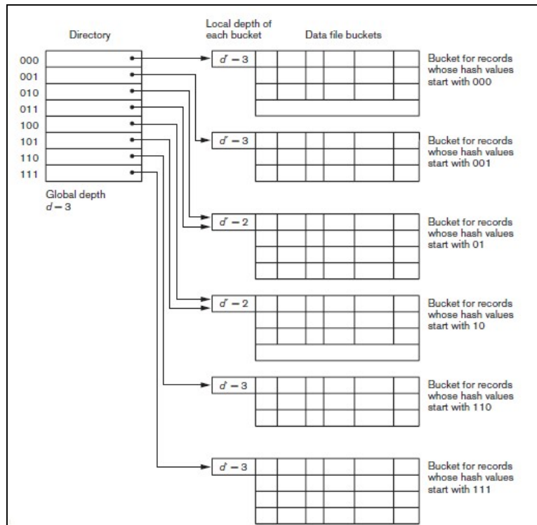
Figure 6.11: Extensible hashing
