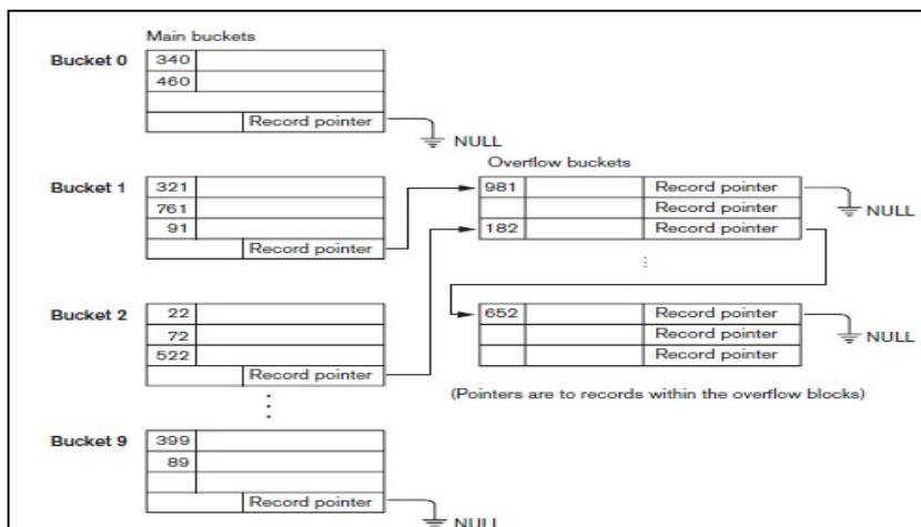
Figure 6.10: Hashing example
