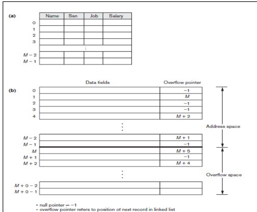
Figure 6.8: Internal hashing
