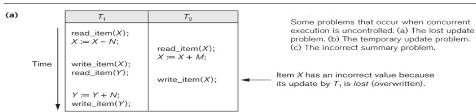
Figure 5.8 (a): Lost update problem
