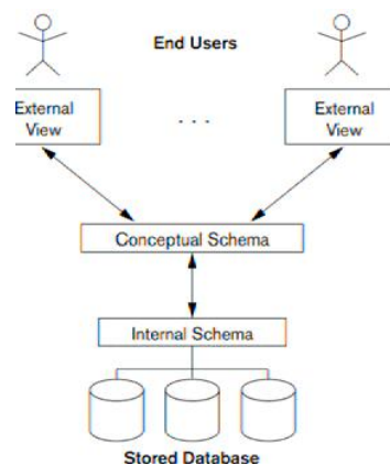
Figure 1.3 The Three Schema Architecture
