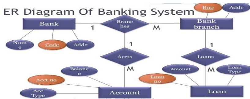
Figure 1.1 ER Diagram of Banking System
