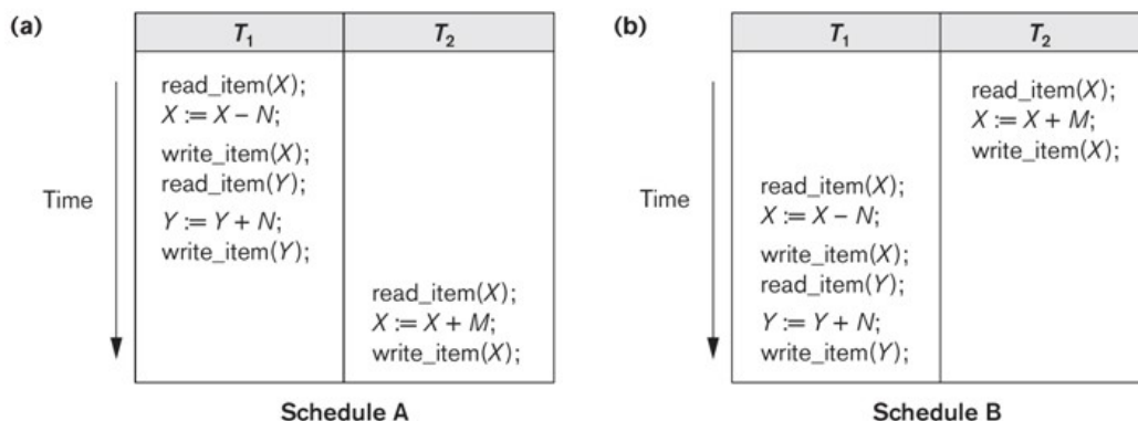
Figure 5.10: Examples of Serial schedules
