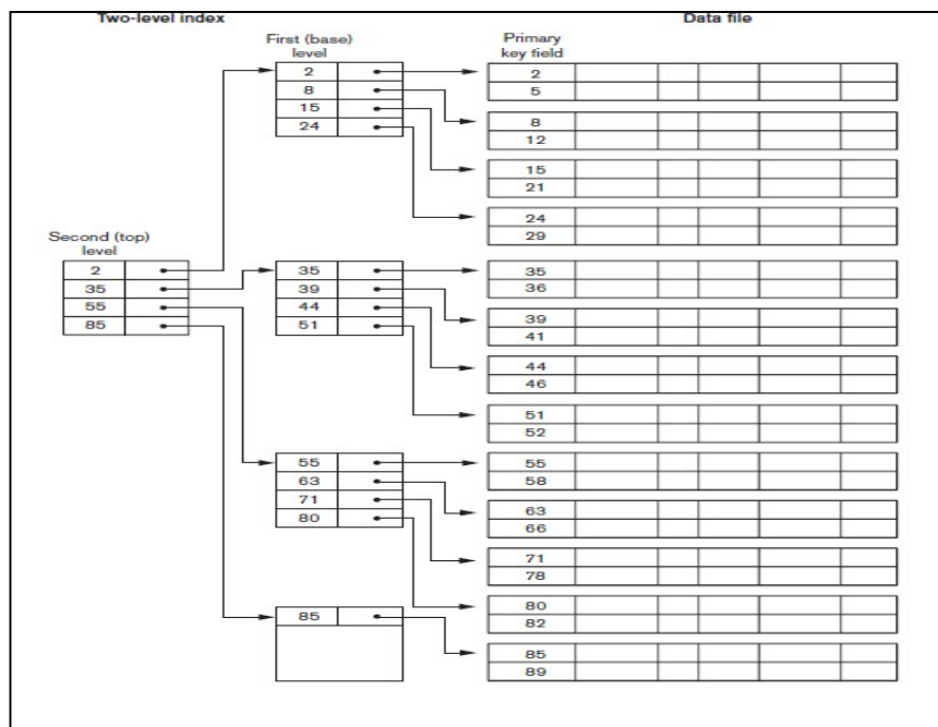
Figure 6.20: Example of secondary index
