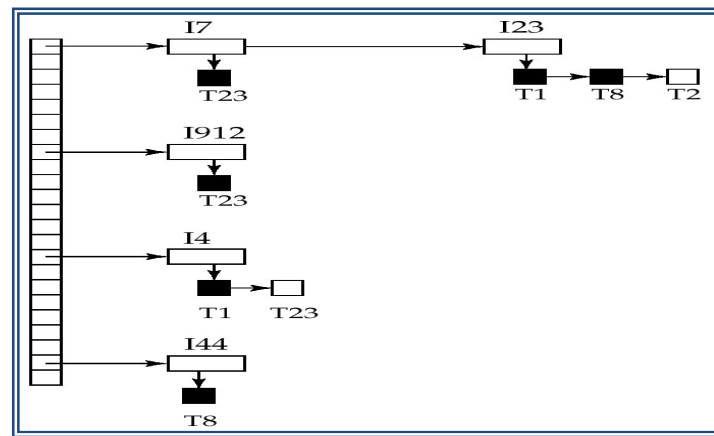
Figure 5.20: Example of Lock table
