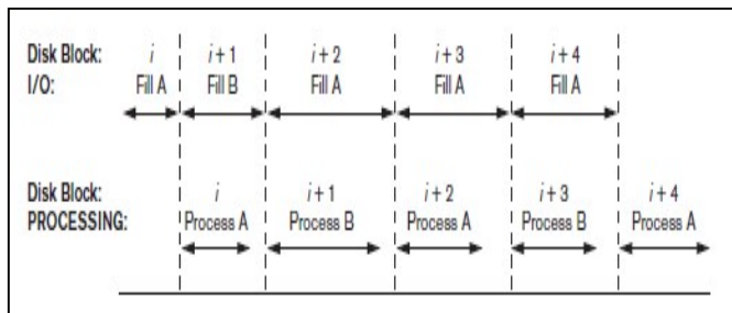
Figure 6.4: Reading and processing can proceed in parallel
