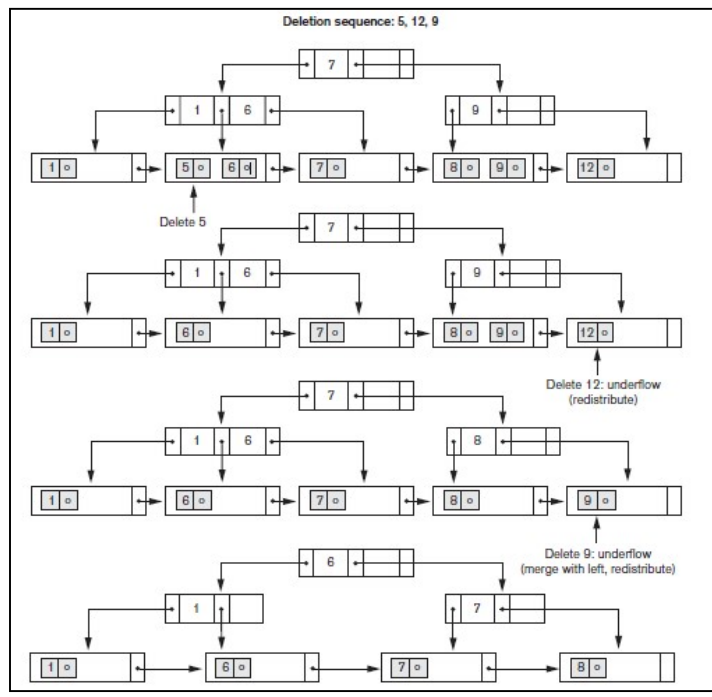
Figure 6.27: Deletion from B+ tree
