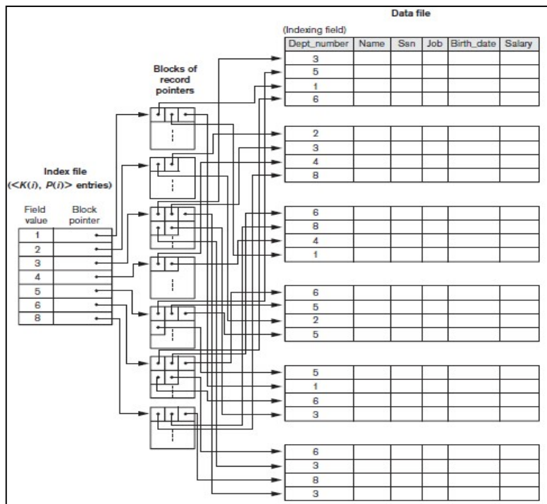
Figure 6.19: Multi level indexes
