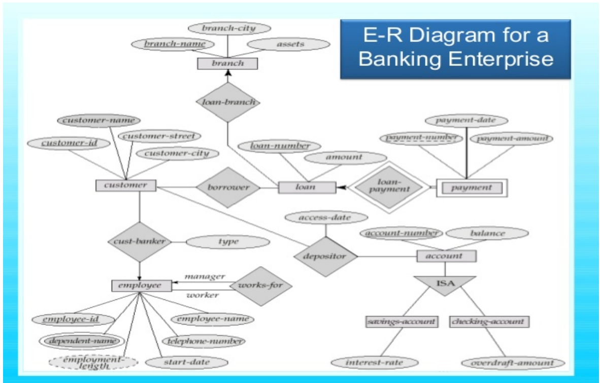
Figure 2.7 E-R diagram of Banking Enterprise System
