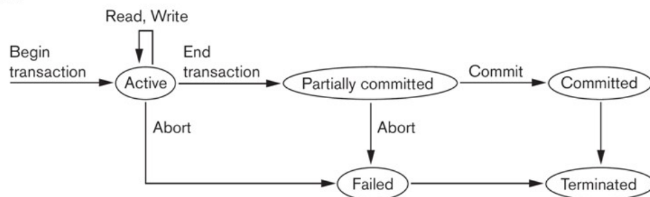
Figure 5.9: State transition diagram of transaction
