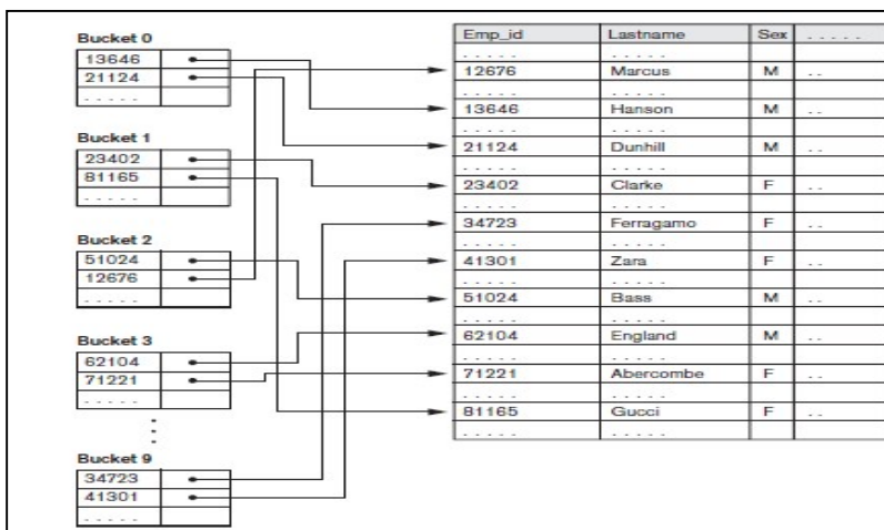
Figure 6.29: Sample Hash index
