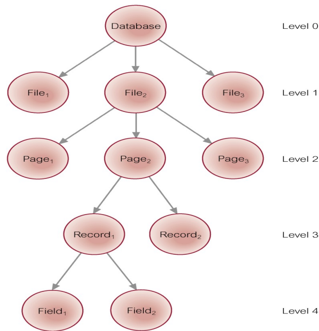
Figure 5.27: Levels of Locking
