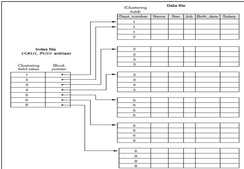
Figure 6.16: Sample clustering index file
