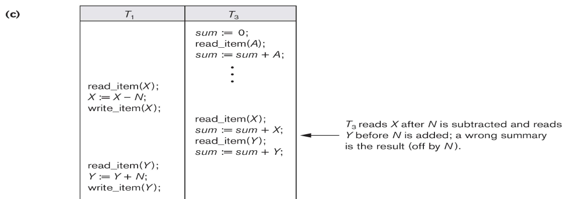
Figure 5.8 (c): Incorrect summary problem
