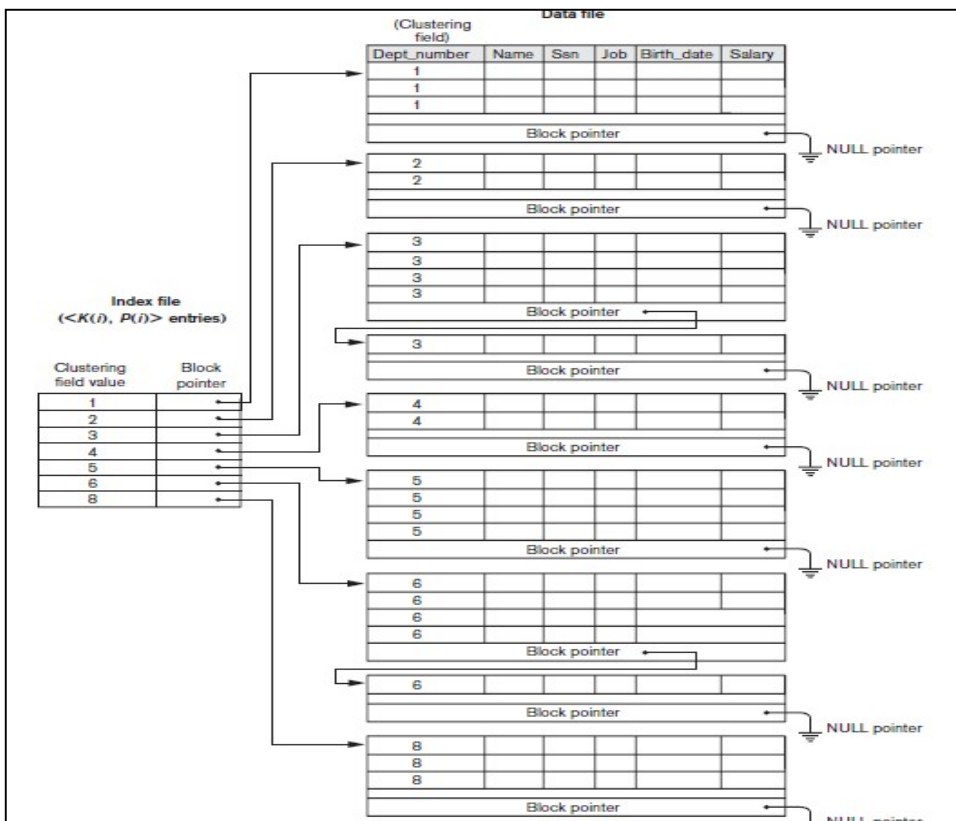
Figure 6.16: Sample clustering index file
