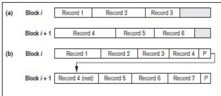
Figure 6.6: Allocating File Blocks on Disk
