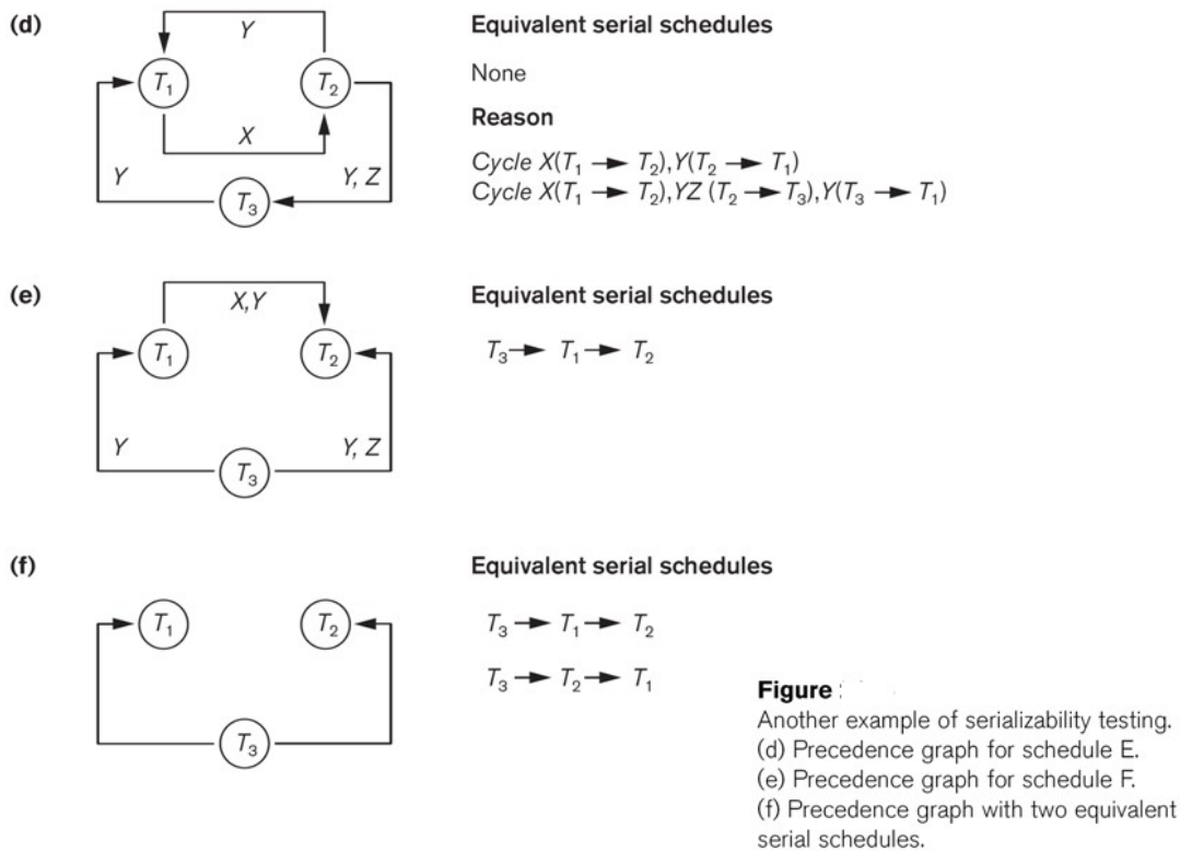
Figure 5.16: Testing for conflict serializability using another example
